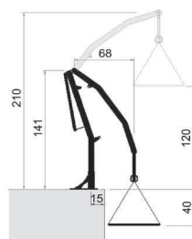
Base atornillable
